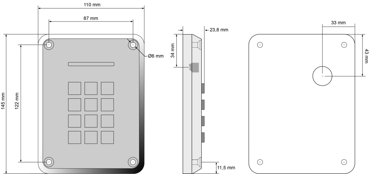
Recommended hole pattern for installation
